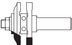
HW STILE AND RAIL ASSEMBLY WITH BALL BEARING GUIDE Z=2 Page 2.25
