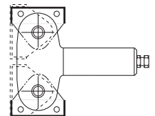
HW INSERT VARI-ANGLE ROUTER CUTTERS 1° Z=2 Page 9.13
