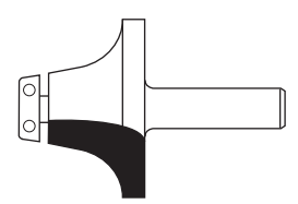
HW ROUNDING OVER UNDERMOUNT BOWL BITS WITH BALL BEARING GUIDE Z=2 Page 3.13
