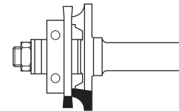
HW BEAD PANELING ASSEMBLY WITH BALL BEARING GUIDE Z=2 Page 2.22
