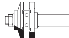
HW STILE AND RAIL ASSEMBLY WITH BALL BEARING GUIDE Z=2 Page 2.24
