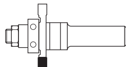
HW TONGUE AND GROOVE ASSEMBLY WITH BALL BEARING GUIDE Z=2 Page 2.24
