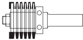
HW FINGER JOINT ASSEMBLY WITH BALL BEARING GUIDE Z=2 Page 2.20
