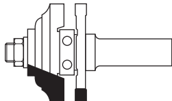
HW STILE AND RAIL ASSEMBLY WITH BALL BEARING GUIDE Z=2 Page 2.26
