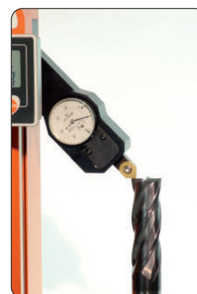
How to measure tool length
