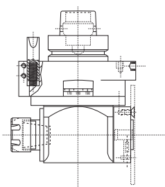
STANDARD TYPE 2-sided angle head 90° (spring collet or sawblade)
