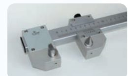
GAUGE FOR LINEAR MEASUREMENTS, DISTANCE FROM THE CENTRES OF THE HOLE TO THE EDGE OF THE PANEL Page 15.14
