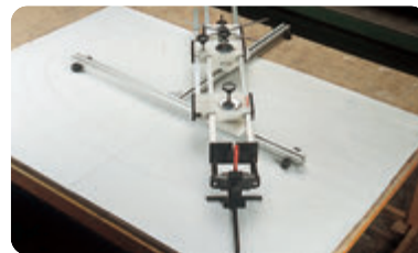
Item ELLISYSTEM “ELLISYSTEM” is the “last born” of our special equipments for producing arch frames. With “ELLISYSTEM” the customer can execute a perfect geometrical ellipse. Suitable for house restoration where the double radius arch is difficult to fit. Simple and easy to use, it keeps the same work procedure and features as “ARKADE” + “ELLIX”
