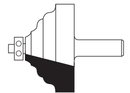
HW EDGE MOULDING BITS WITH BALL BEARING GUIDE Z=2 Page 3.11
