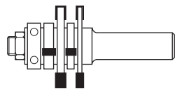
HW SLOT CUTTER SET WITH BALL BEARING GUIDE Z=2 Page 2.21
